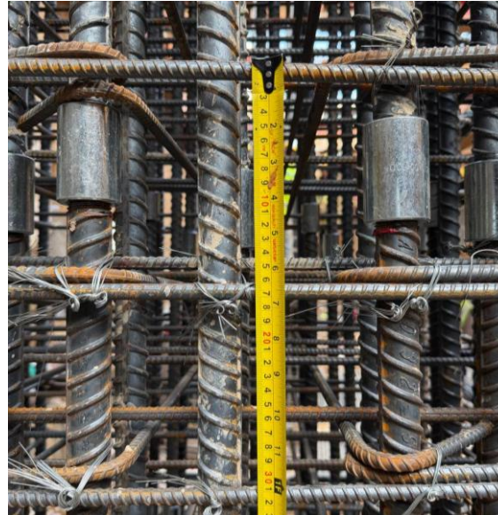
Check spacing of Tie
