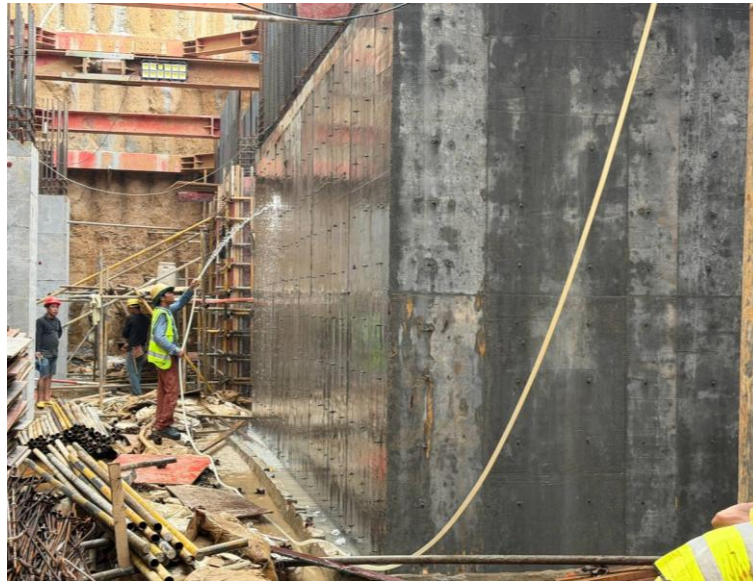
Curing of Concrete
