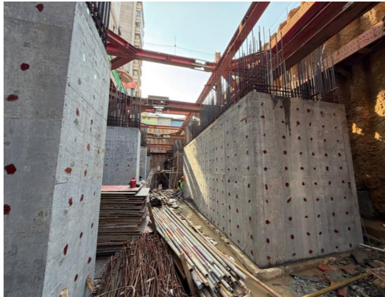
Concrete of Core Walls
