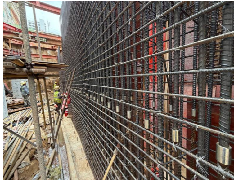
Inspection of Rebar of Core Walls
