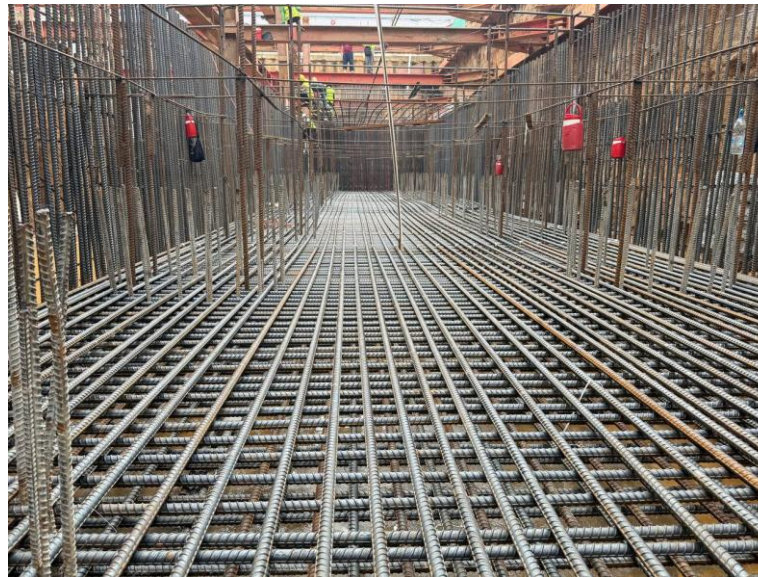
Inspection of Bottom and Side bar of PC4
