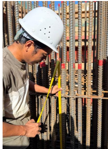
Inspection of starter rebar of columns
