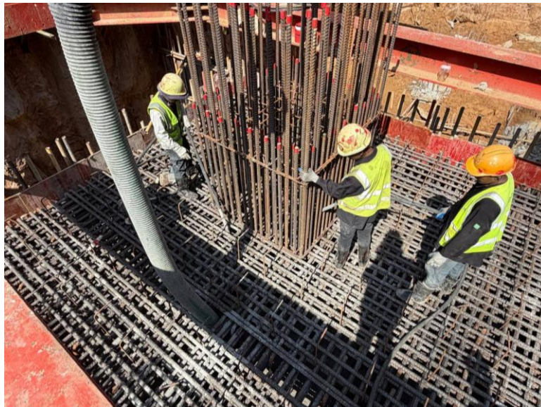
Casting concrete of PC4
