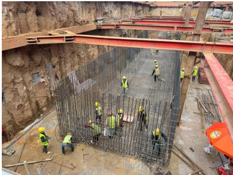
Install Bottom and Side bars of PC4
