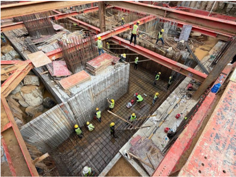
Install rebar of Septic Tank
