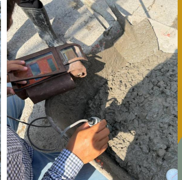
Check Cl- content
