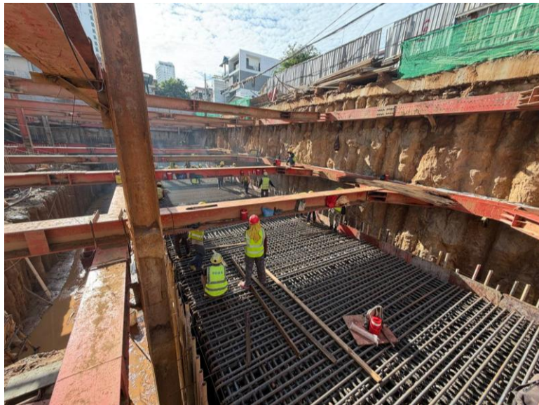
Install Top and Hook bars of PC4
