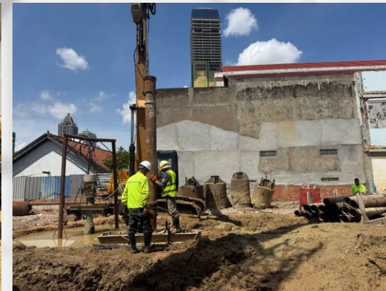
Inserting trimie pipe.
